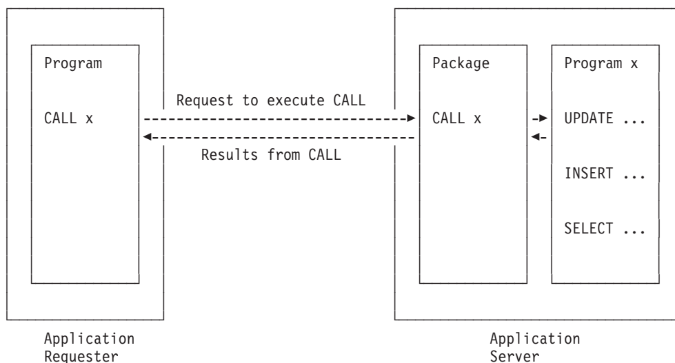
Figure 2. Application with remote procedure
