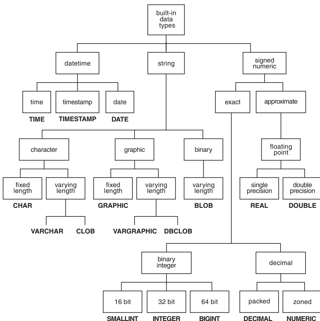
Figure 9. Data Types Supported by the DB2 Relational Database Products
